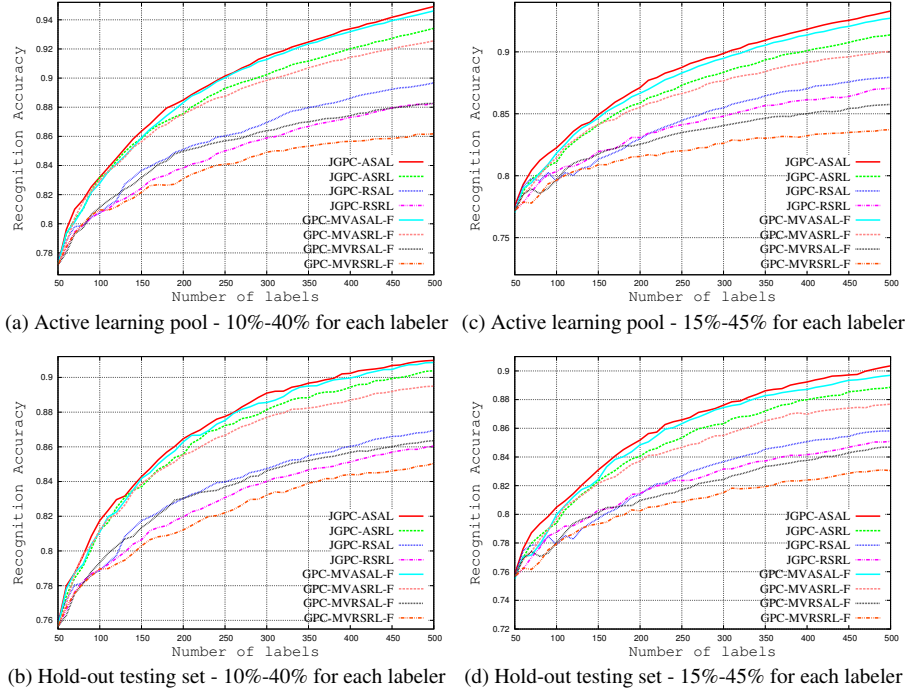
Figure 4: Experiments with labelers with different level of label noises on the ImageNet dataset: (a)&(b) Each labeler is simulated with 10%, 15%, 20%, 25%, 30%, 35% and 40%, respectively; (c)&(d) Each labeler is simulated with 15%, 20%, 25%, 30%, 35%, 40%, and 45%, respectively.
