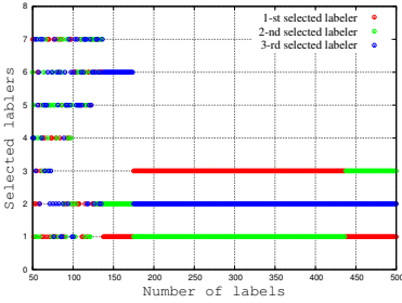
Figure 3: Selected labelers on “Meerkat, meerkat” class with 4 bad labelers.
